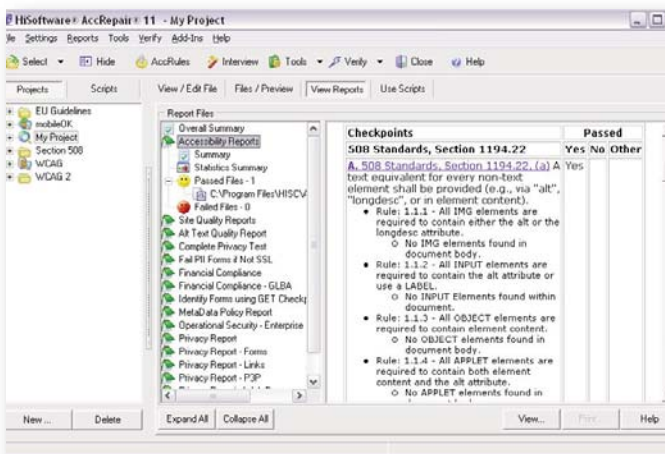
Above left: Project View
